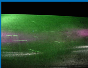
Drive Shaft with Heat Treatment Induced Cracks
