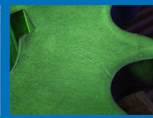
Gear with Service Induced Crack
