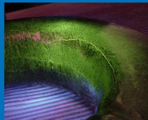
Crane Hook with Service Induced Crack
