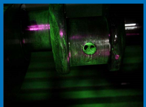
Crank Shaft with Service Induced Crack Near Lube Hole
