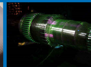
Splined Shaft with Service Induced Cracks
